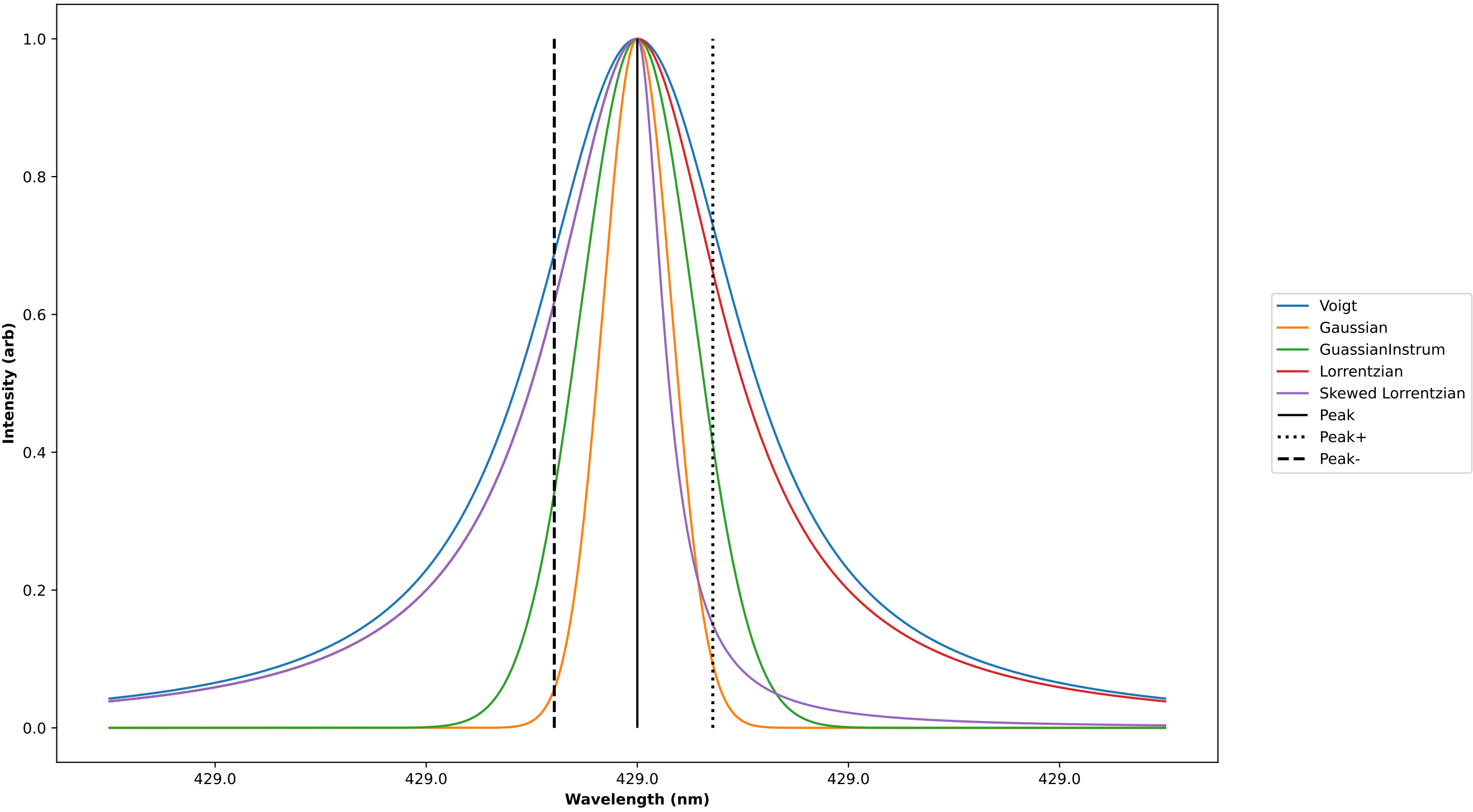
Comparing all Lineshapes without Doppler
